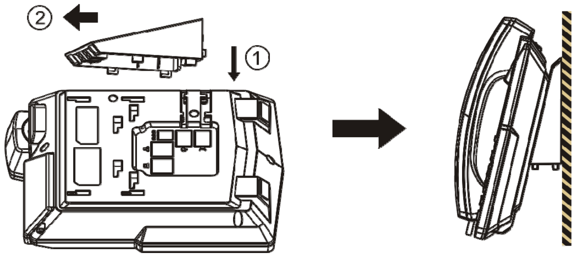
Figure 2 - Wall-mount Installation
